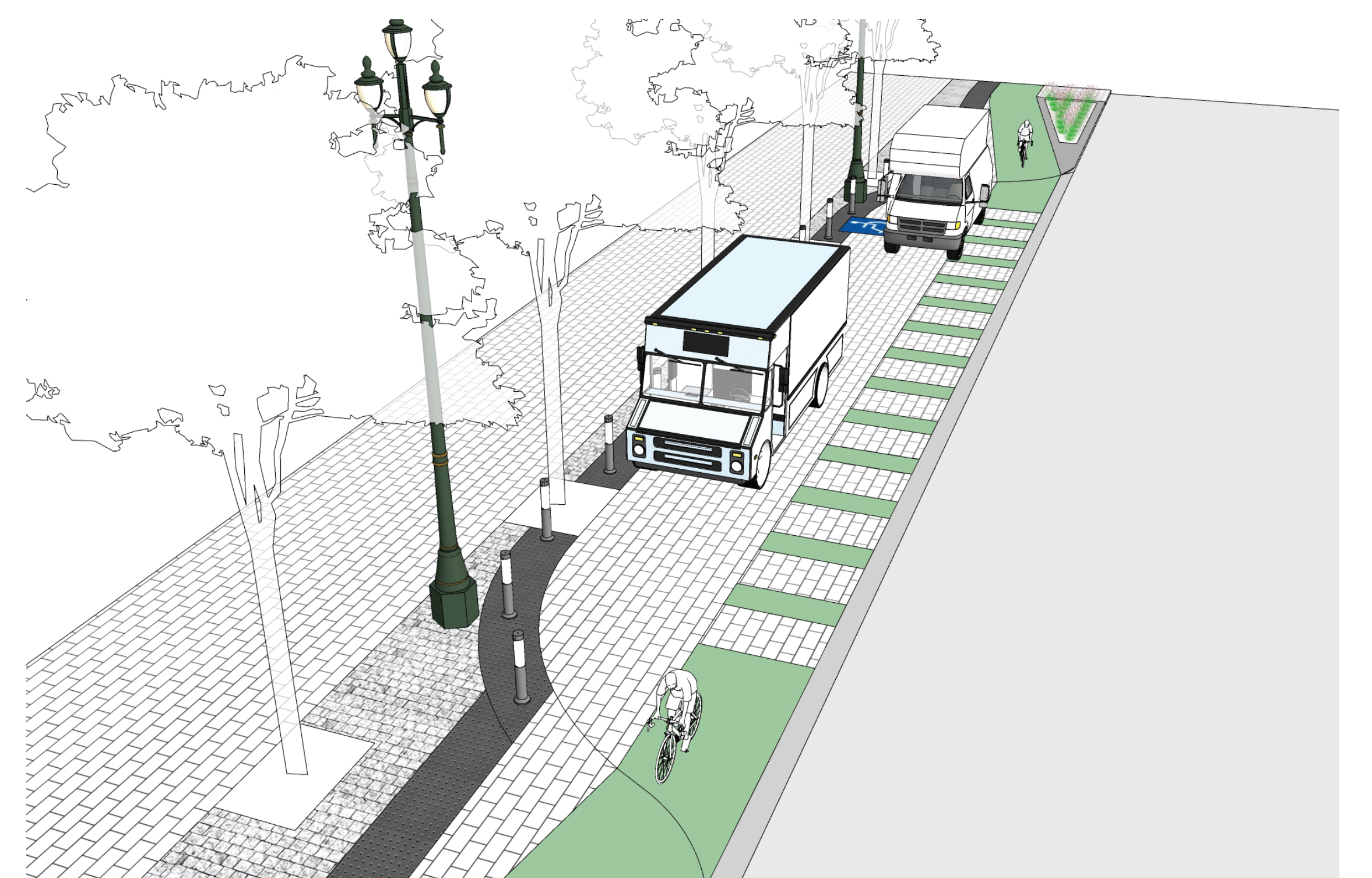
Proposed sidewalk-level bikeway design at commercial loading zones on Market
